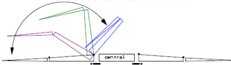
SYSTEM OPENING/CLOSING 12 MT. OS BOOM 2 RAMS
